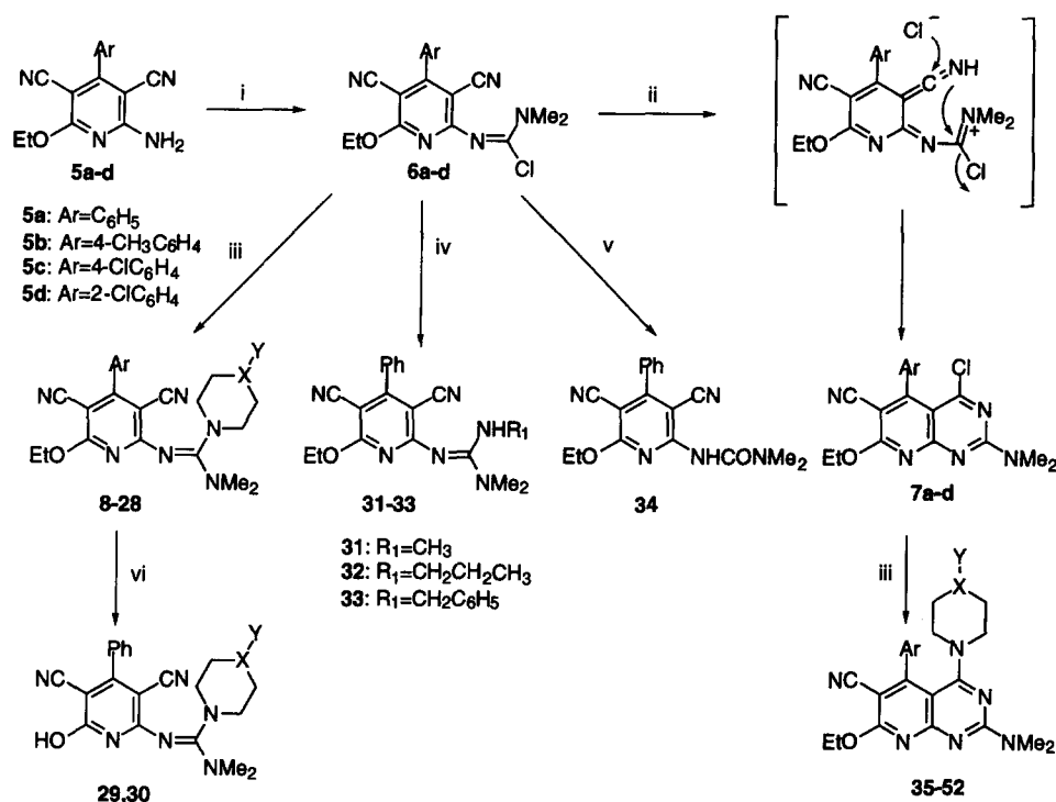
Scheme 1. (i) Cl 2 CN + Me 2 Cl - , 1,2-dichloroethane, reflux, 20 h; (ii) HCl (g) , 1,2-dichloroethane, rt; (iii) secondary amine, ethanol, reflux; (iv) primary amine, ethanol, reflux; (v) NH 4 OH, acetonitrile, rt; (vi) NaOH, ethanol, reflux.
